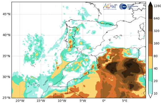
Barcelona Dust Forecast Center - http://dust.aemet.es/ NMMB-MONARCH Res:0.1°x0.1° Dust Surface Conc. ( \mu\text{g}/\text{m}^3 ) Run: 12h 28 FEB 2021 Valid: 00h 02 MAR 2021 (H+36)
