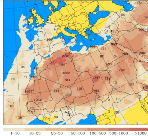
University of Athens (AM&WFG) SKIRON Forecast Dust Concentration Near Ground ( \mu\text{g}/\text{m}^3 ) Tue 02.03.21 at 12 UTC
