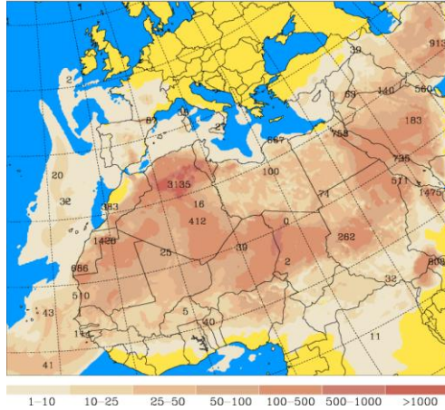
University of Athens (AM&WFG) SKIRON Forecast Dust Concentration Near Ground ( \mu\text{g}/\text{m}^3 ) Tue 02.03.21 at 00 UTC
