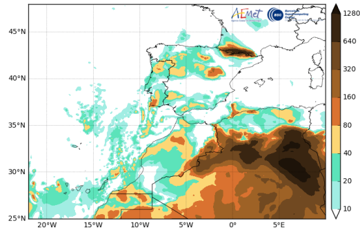
Barcelona Dust Forecast Center - http://dust.aemet.es/ NMMB-MONARCH Res:0.1°x0.1° Dust Surface Conc. ( \mu\text{g}/\text{m}^3 ) Run: 12h 28 FEB 2021 Valid: 12h 02 MAR 2021 (H+48)
