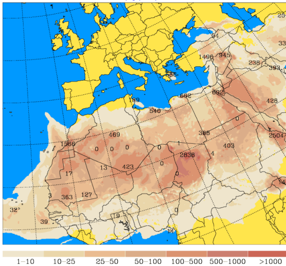
University of Athens (AM&WFG) Dust Concentration Near Ground ( \mu\text{g}/\text{m}^3 )
