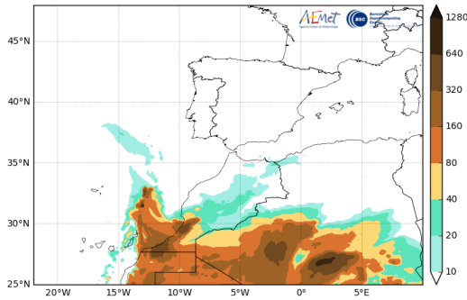
Barcelona Dust Forecast Center - http://dust.aemet.es/ NMMB-MONARCH Res:0.1°x0.1° Dust Surface Conc. ( \mu\text{g}/\text{m}^3 ) Run: 12h 13 DEC 2021 Valid: 00h 15 DEC 2021 (H+36)
