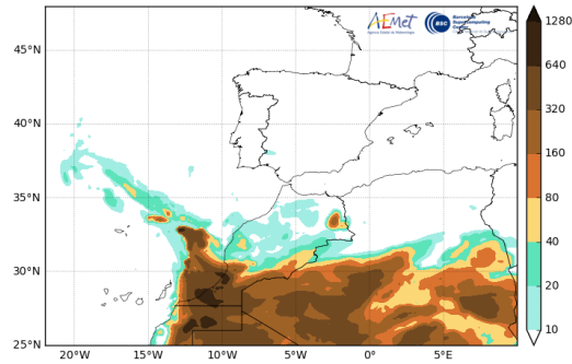
Barcelona Dust Forecast Center - http://dust.aemet.es/ NMMB-MONARCH Res:0.1°x0.1° Dust Surface Conc. ( \mu\text{g}/\text{m}^3 ) Run: 12h 13 DEC 2021 Valid: 12h 15 DEC 2021 (H+48)
